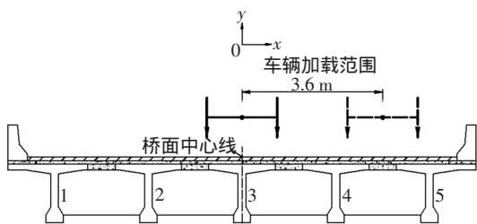
图 5 车辆的横向加载范围 Fig.5 The allowable range for transverse truck position
